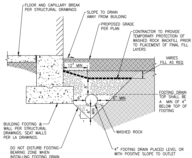
INTERCEPTOR/WALL DRAIN NTS 2
