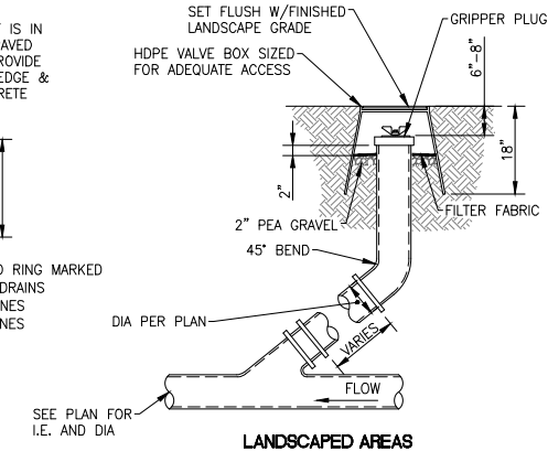
LANDSCAPED AREAS
