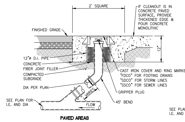
PAVED AREAS
