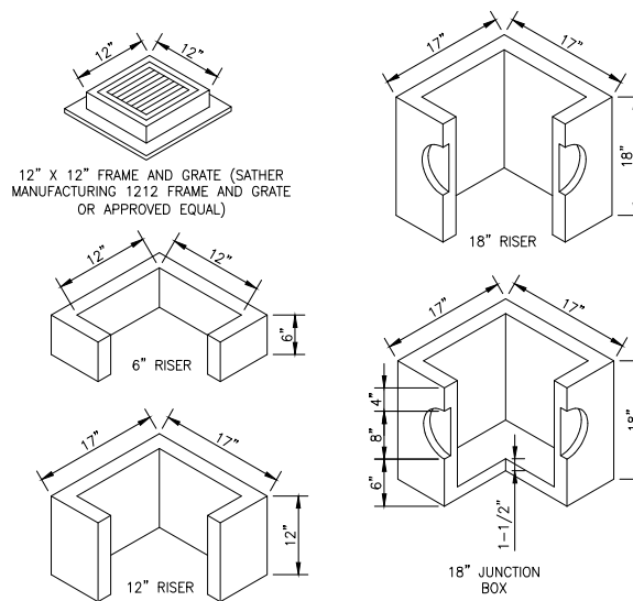
17" X 17" AREA DRAIN BY CUZ CONCRETE PRODUCTS OR EQUAL
