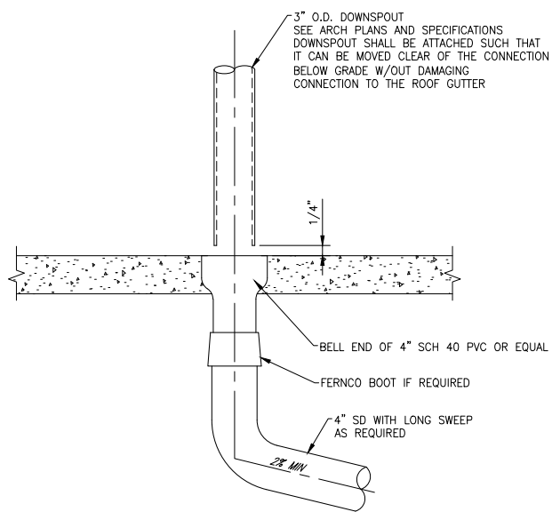
RESIDENTIAL ROOF DOWNSPOUT NTS 9
