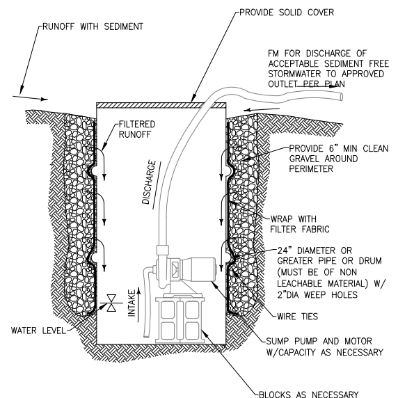
NTS MOVEABLE SUMP & PUMP 2
