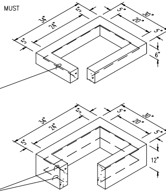
1 #3 BAR HOOP
